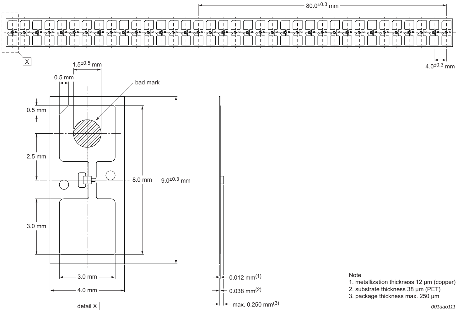
Fig 9. Package FCS2, SOT1040AA1, 12 \mu m Cu metallization
